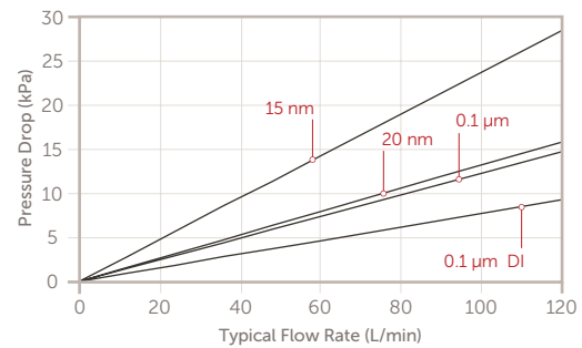
Trinzik UPW 30" Cartridges
