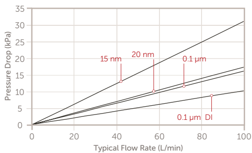
Trinzik UPW 20" Cartridges
