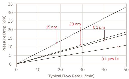
Trinzik UPW 10" Cartridges
